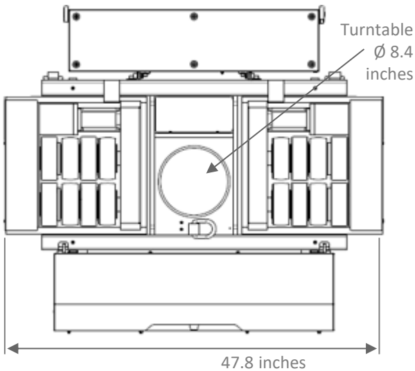
Side Views
